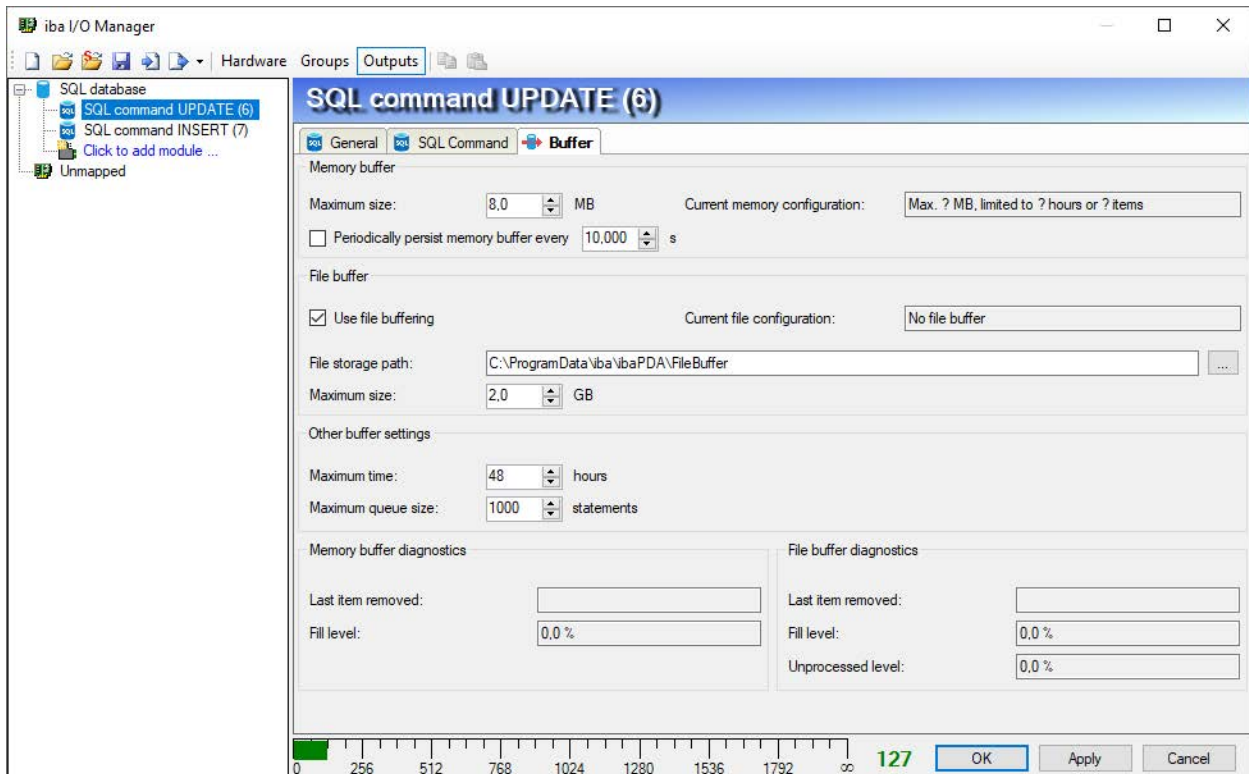
Fig. 8: Configuration of buffering, example SQL-Server
