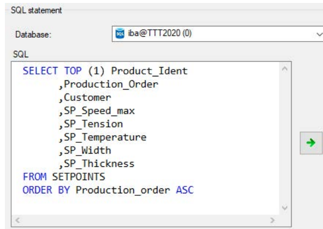
Fig. 9: Example of an SQL query
