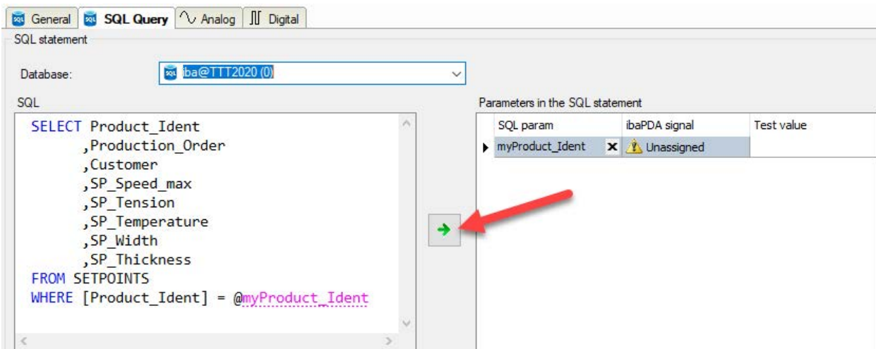
Fig. 13: Example SQL query depending on the product ID with a parameter “myProduct_Ident”
