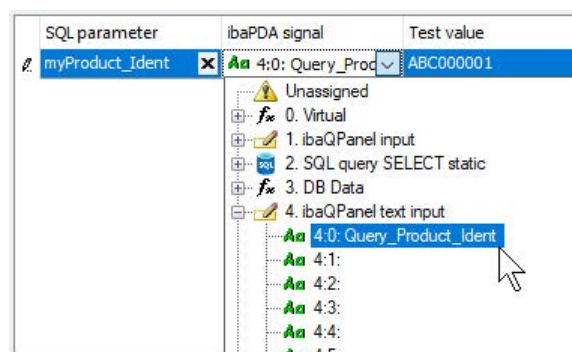
Fig. 14: Assignment of parameter and signal
