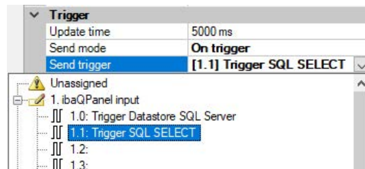
Fig. 7: Example of a DB query depending on a QPanel input
