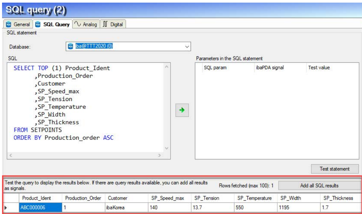
Fig. 10: Result of the test query
