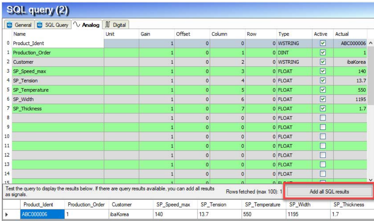
Fig. 11: Example of the query of a value series (the first) from a table with 8 columns
